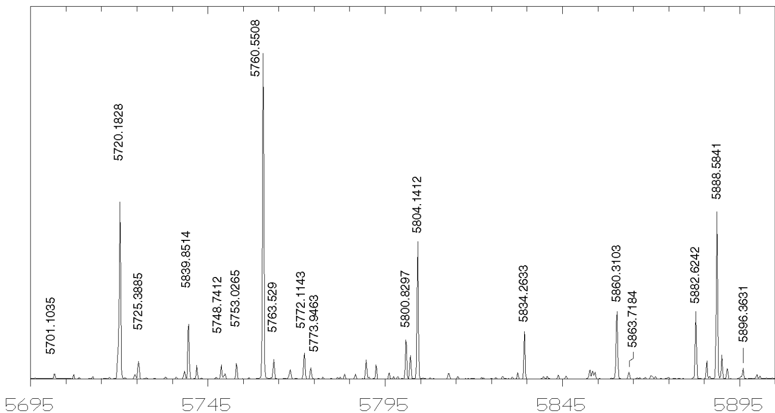
NAO Rozhen ThAr comparison spectrum (R=18000; I=4 mA)
